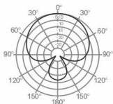
Polar Pattern
